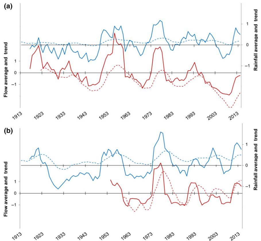
FIGURE 2 Annual averages and trends in rainfall (blue) and flows (red) in the developed Murray–Darling Basin and the undeveloped Lake Eyre Basin, 1913–2014. Long-term 5-year moving annual averages of standardized (z-score) rainfall and river flows (continuous lines) and their cumulative, 10-year annual trend (adding these 5 year averages; dashed lines) for (a) the developed Murray–Darling Basin and (b) the undeveloped Lake Eyre Basin. [Color figure can be viewed at wileyonlinelibrary.com ]
